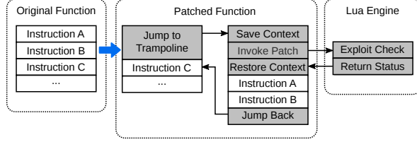
Figure 8: Live patching through function hooking
