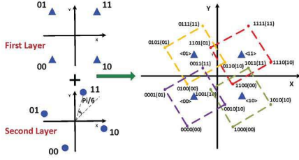
Fig. 3: An Example for Permit Symbol Constellation
