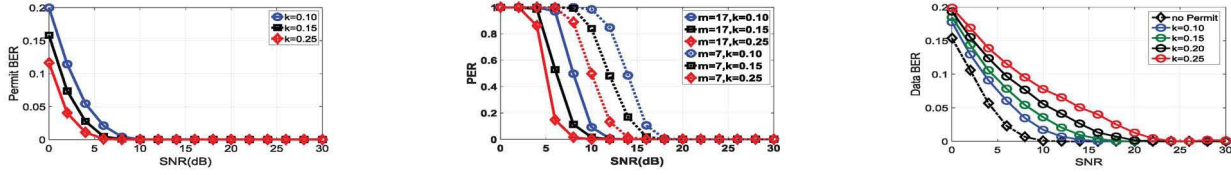
(a) Permit BER vs. SNR with m = 17
