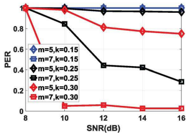
Fig. 12: PER Performance using USRP
