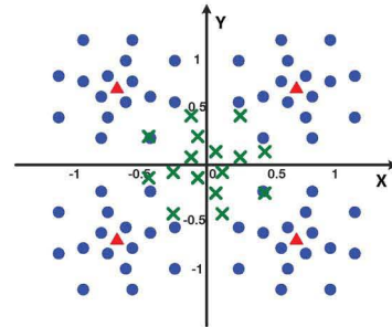
Fig. 6: Constellation of the Transmitted Symbols
