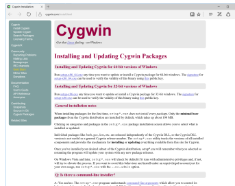
Figure 13: Installing Cygwin
