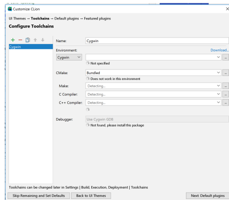
Figure 12: Toolchains
