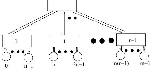
Fig. 2. The subgraph of ftree(n+m, r) ( ftree(n+1, r) )
