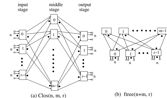
Fig. 1. Clos and folded-Clos networks
