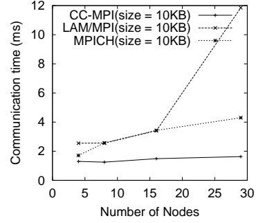
Figure 8: Performance of MPI_Bcast (size=10KB).
