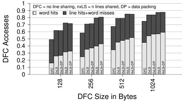
Fig. 14. DFC Data Hit Rates
