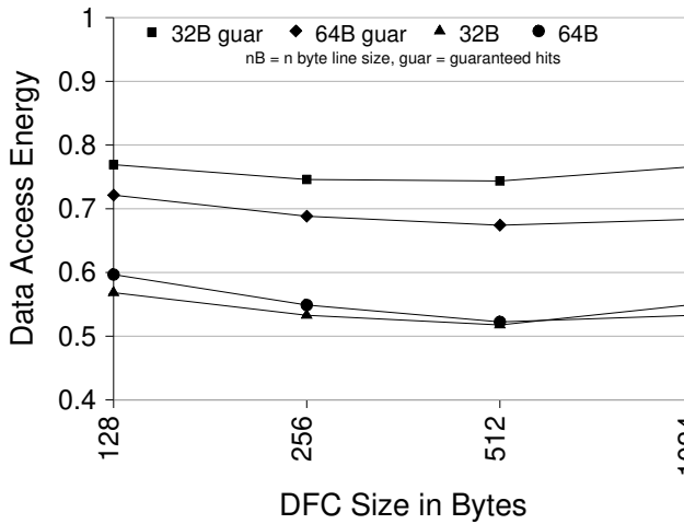
Fig. 19. Data Access Energy with Guaranteed DFC Hits
