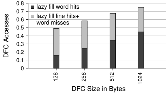
Fig. 10. Taxonomy of DFC Accesses
