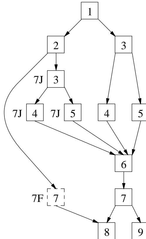
Restructured Control Flow
