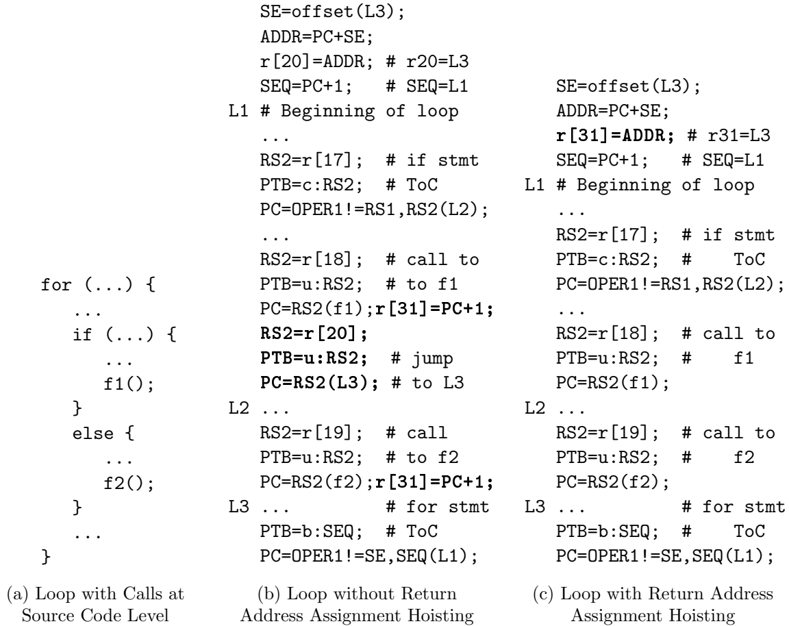
Figure 3.7: Example of Return Address Assignment Hoisting
