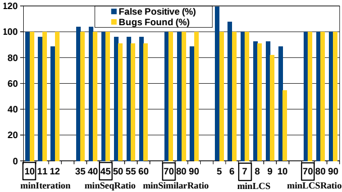
Fig. 12. Parameter-sensitivity experiments. Each configuration changes only one threshold, with its value shown on the X-axis. The default values are boxed. Two sets of experiments are conducted for each configuration: the left/dark bar shows false positives on JUnit tests, and the right/light bar shows bugs found on bug-triggering inputs. The Y-axis shows the numbers normalized to the results under default setting.
