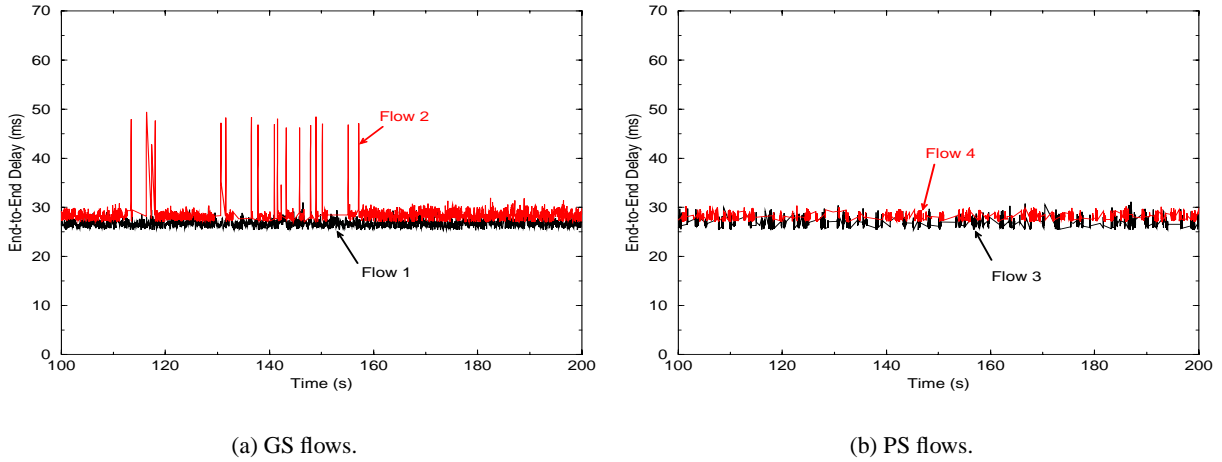
Figure 16: End-to-end packet delays of the GS/PS flows in path traversing G1(s) to G1(D) in the chain network.
