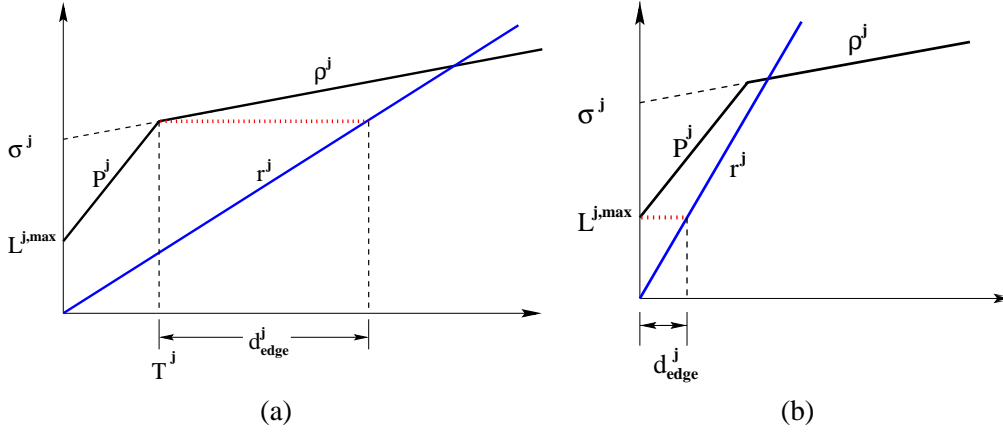
Figure 4: Edge node shaping and marking for an GS flow.
