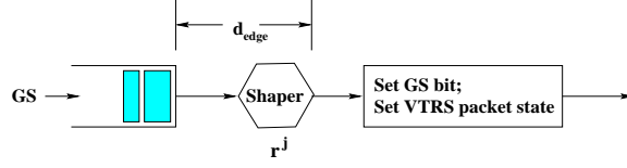
Figure 4: Edge node shaping and marking for an GS flow.
