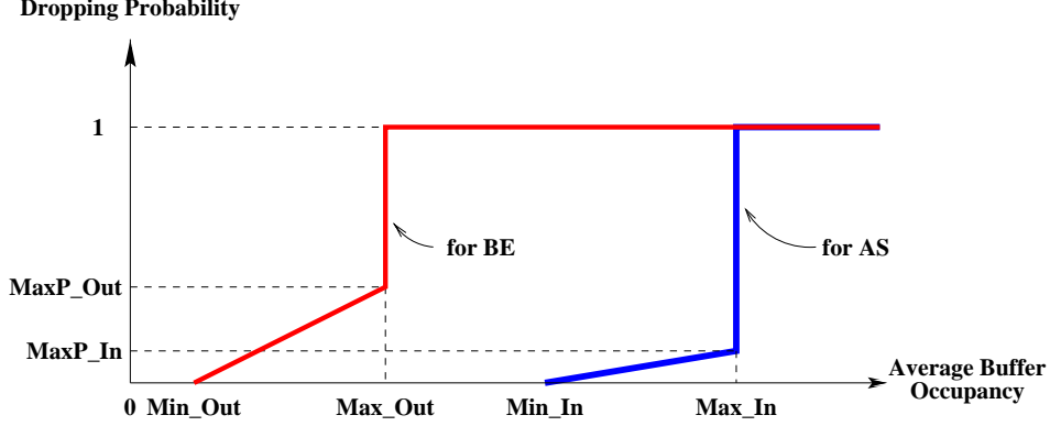
Figure 9: Buffer management for the AS and the BE traffic with RIO mechanism.
