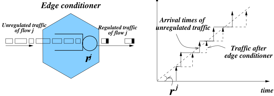
Figure 2: Edge conditioning and its effect in the VTRS.
