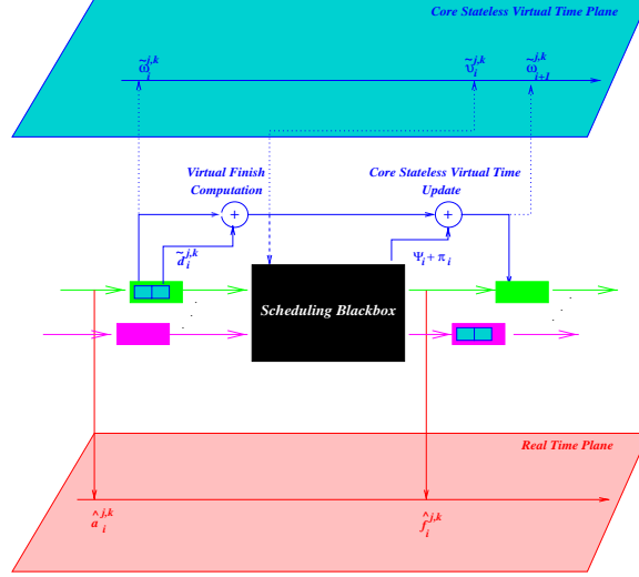
Figure 3: Per-hop behavior and operations at a core node under the VTRS.
