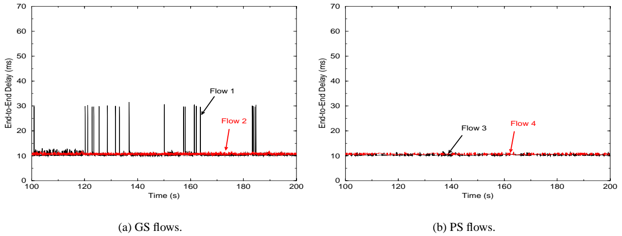
Figure 14: End-to-end packet delays of the GS/PS flows in path traversing G1(s) to G1(D) in the peer-to-peer network.
