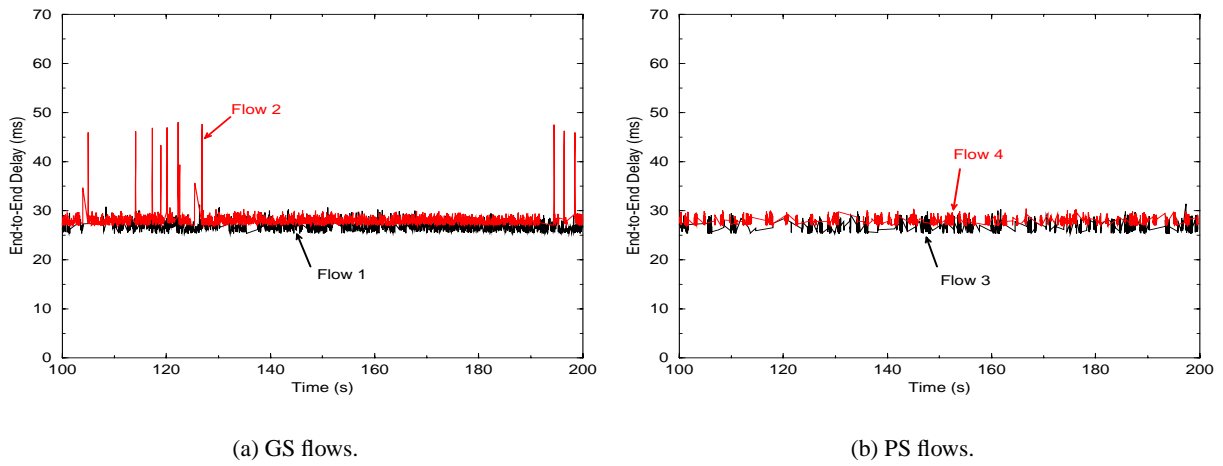
Figure 15: End-to-end packet delays of the GS/PS flows in path traversing G1(s) to G1(D) in the parking-lot network.
