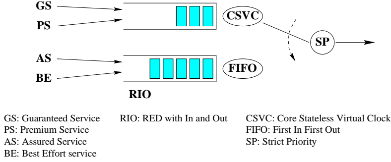
Figure 8: A stateless node architecture for integrated support of the GS, the PS, the AS, and the BE services.
