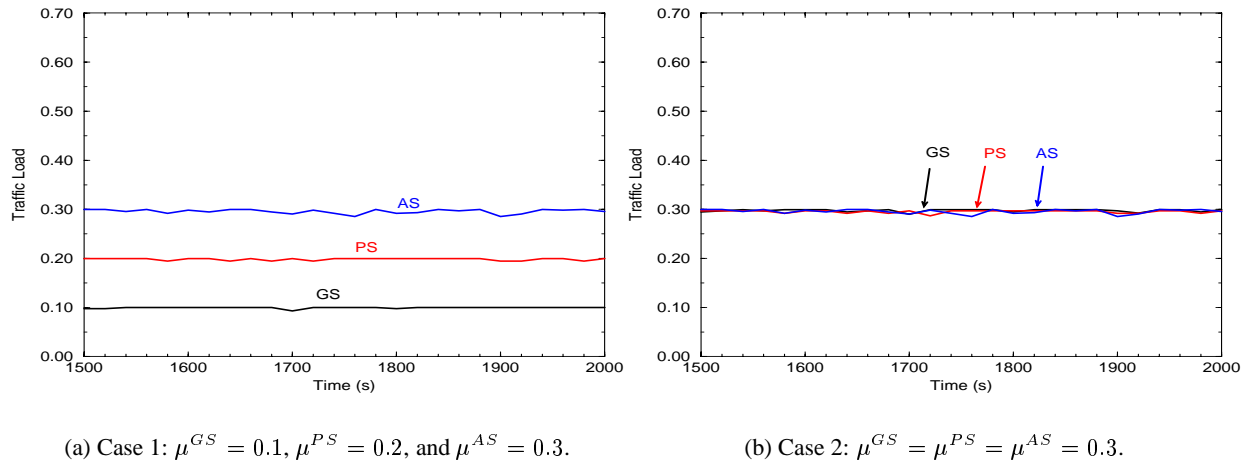
Figure 17: Traffic load on the link between ingress and egress nodes for each type of services in the peer-to-peer network.
