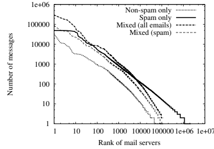
Fig. 6. Rank of mail servers based on # of messages.
