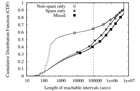
Fig. 13. Network reachable intervals.
