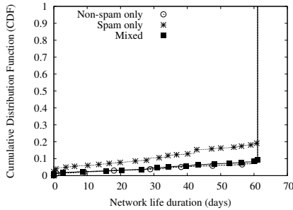
Fig. 11. Network life duration.
