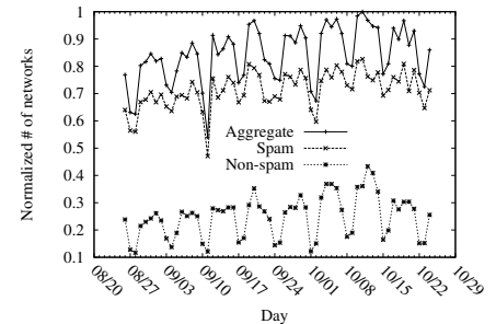
Fig. 4. Normalized daily # of networks (max # of networks = 22, 968).
