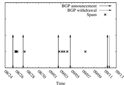
Fig. 14. Spamming correlated with BGP updates (62.215.96.0/19).
