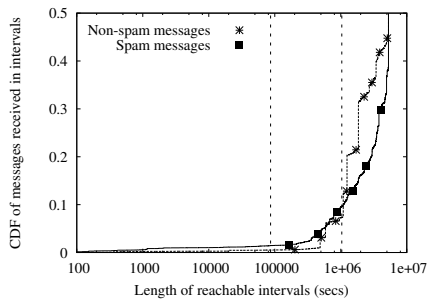
Fig. 15. Email arrivals in different network reachable intervals.
