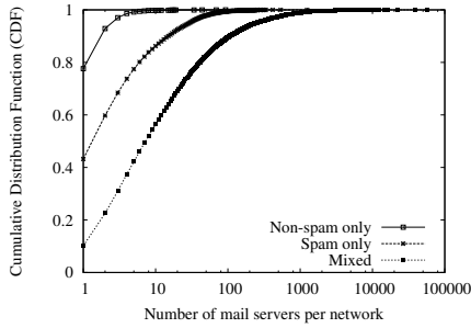
Fig. 8. Number of mail servers of each network.
