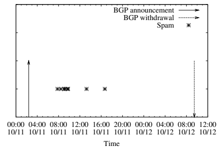
Fig. 12. Spam network with short life duration (222.46.32.0/20).
