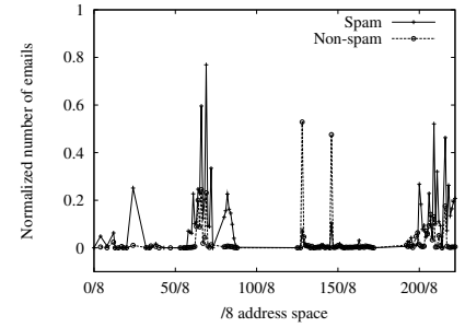
Fig. 7. Normalized number of messages from each “/8” address space.
