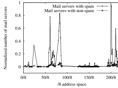
Fig. 9. Normalized # of mail servers of each “/8” address space.
