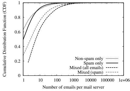
Fig. 5. # of emails from each mail server.
