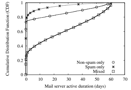
Fig. 10. Mail server active duration (days).
