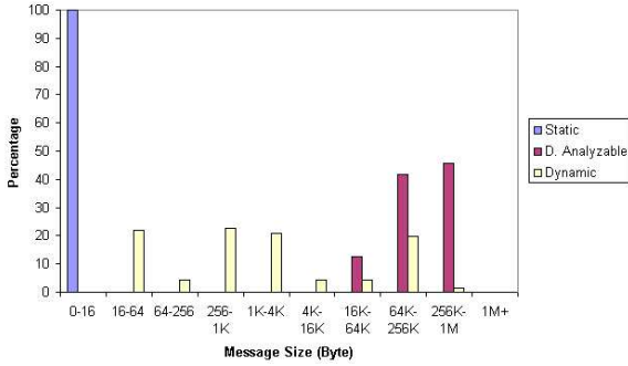
Fig. 3. Message size distribution for point-to-point communications
